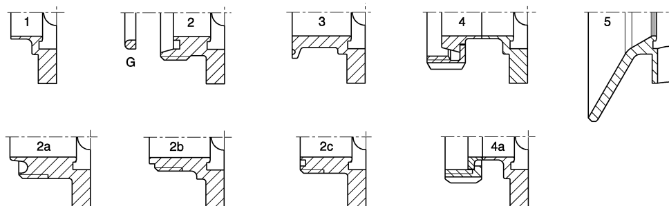
Fig.2: Two-piece flange versions
