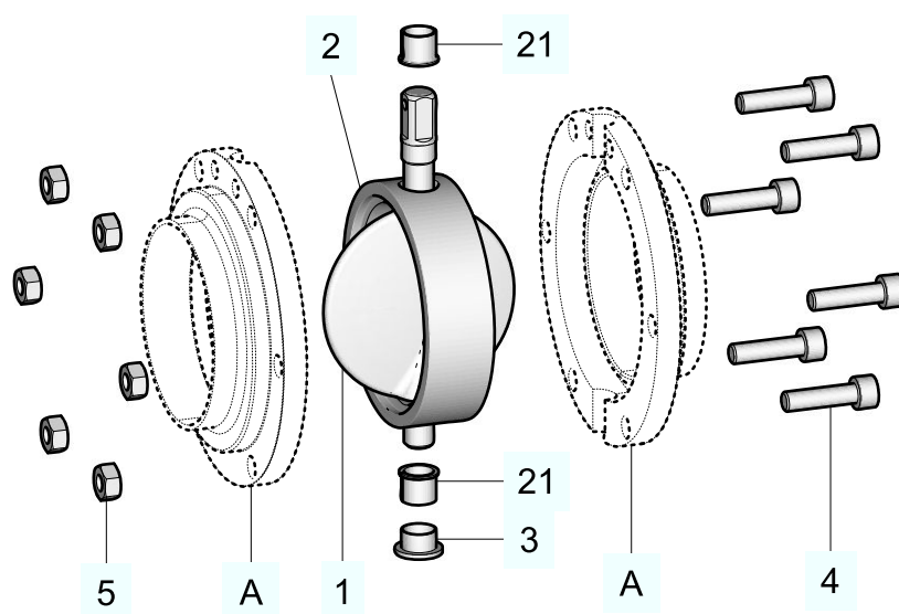
Fig.1: Butterfly valve body T-smart 7
