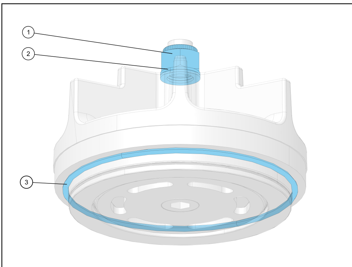
Figure 2-13 - DISCHARGE VALVE
