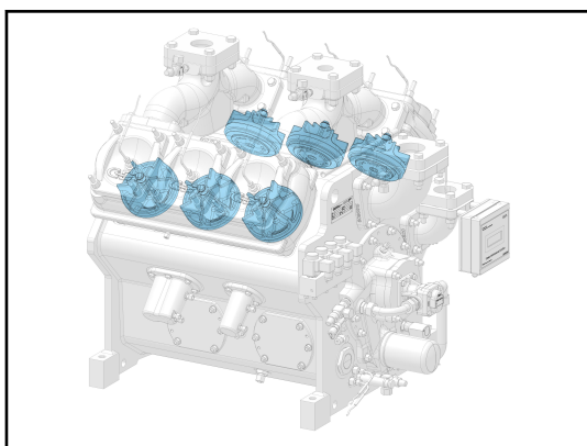
Figure 2-12 - DISCHARGE VALVE
