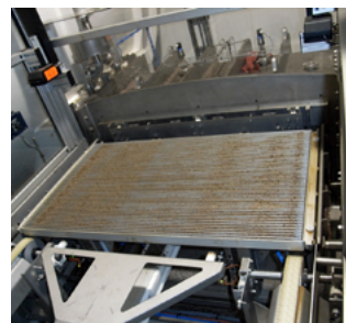
4. Freeze drying – tray going into the Atlas CONRAD® freeze dryer
