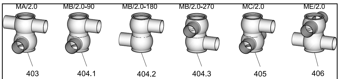
Figure 3-1 - Spare parts - mixproof valve 24/7 PMO M/2.0 with cleaning of lower balancers
