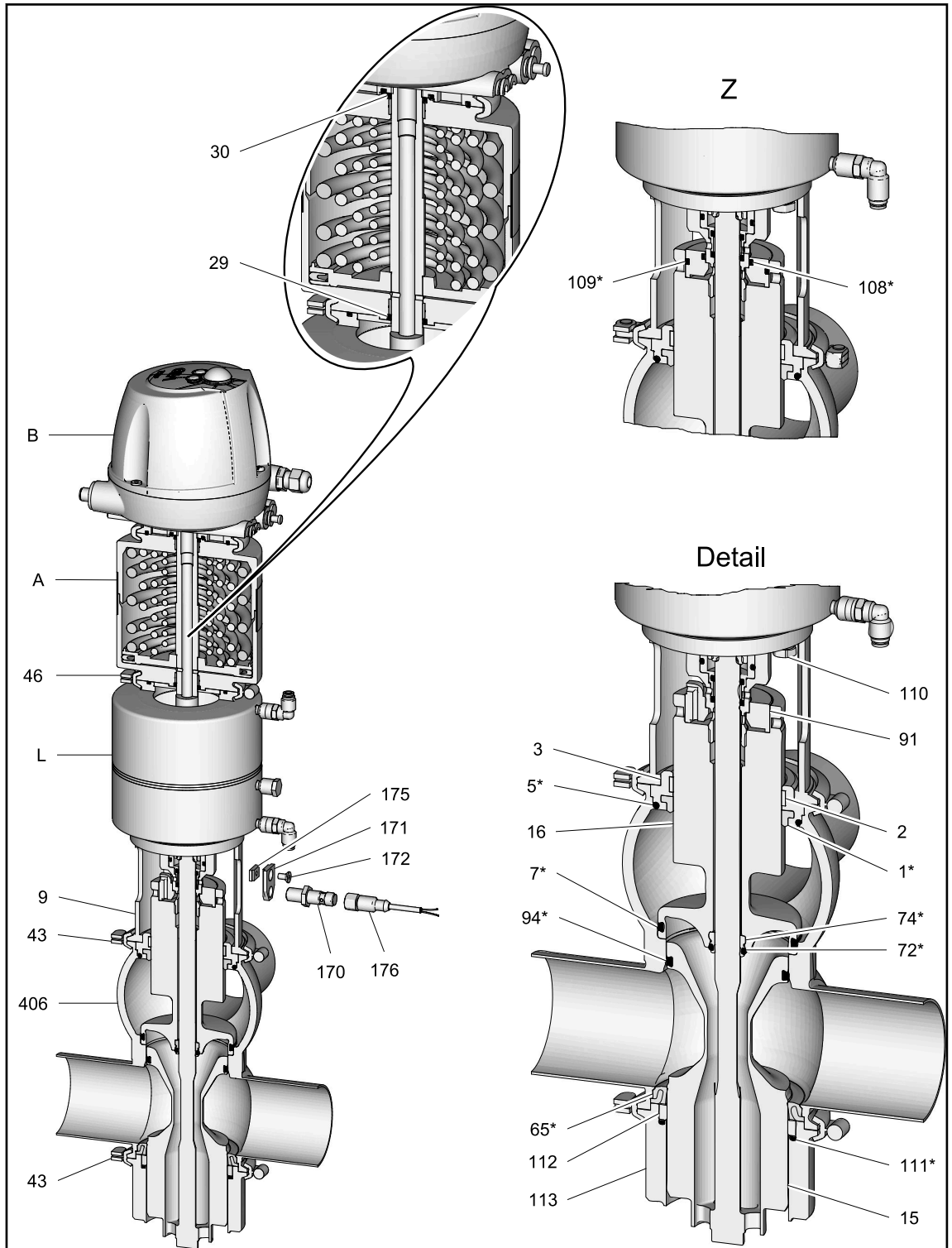
Figure 3-1 - Spare parts - mixproof valve 24/7 PMO M/2.0 with cleaning of lower balancers
