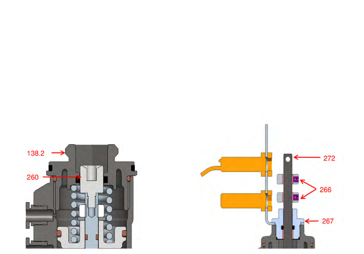
Plastic and stainless-steel actuator with T-VIS
