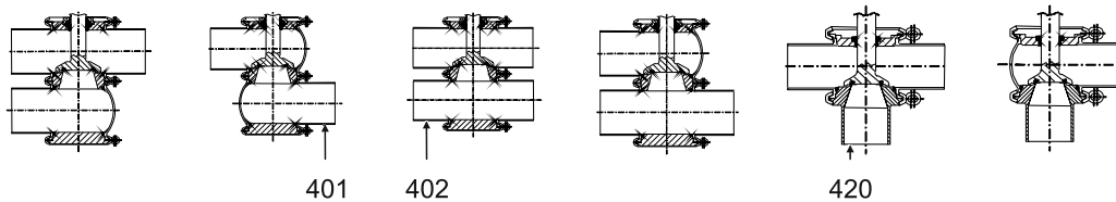
Housing combinations
