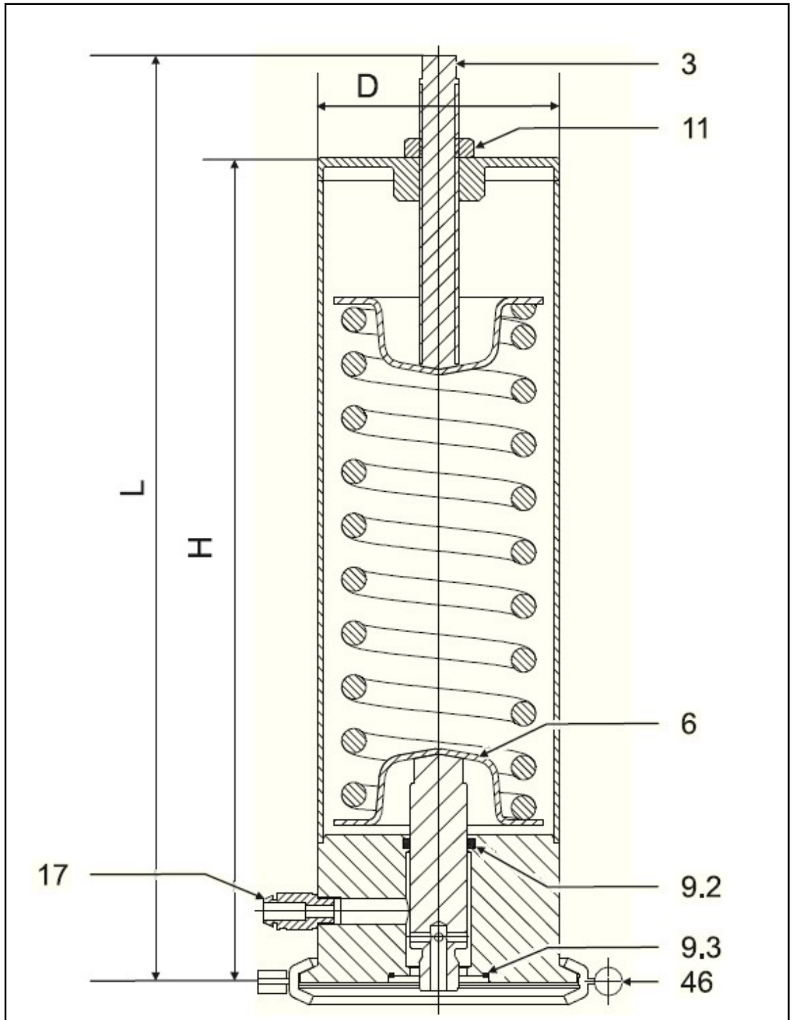
Figure 1 - Actuator F-CJ - only use in connection with actuator CJ.
