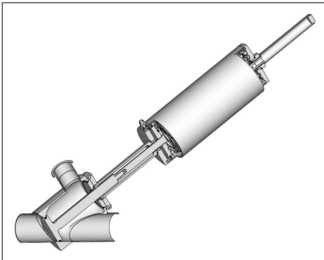
Figure 3-2 - Spare parts - Valve NI / ECO with CIP connection
