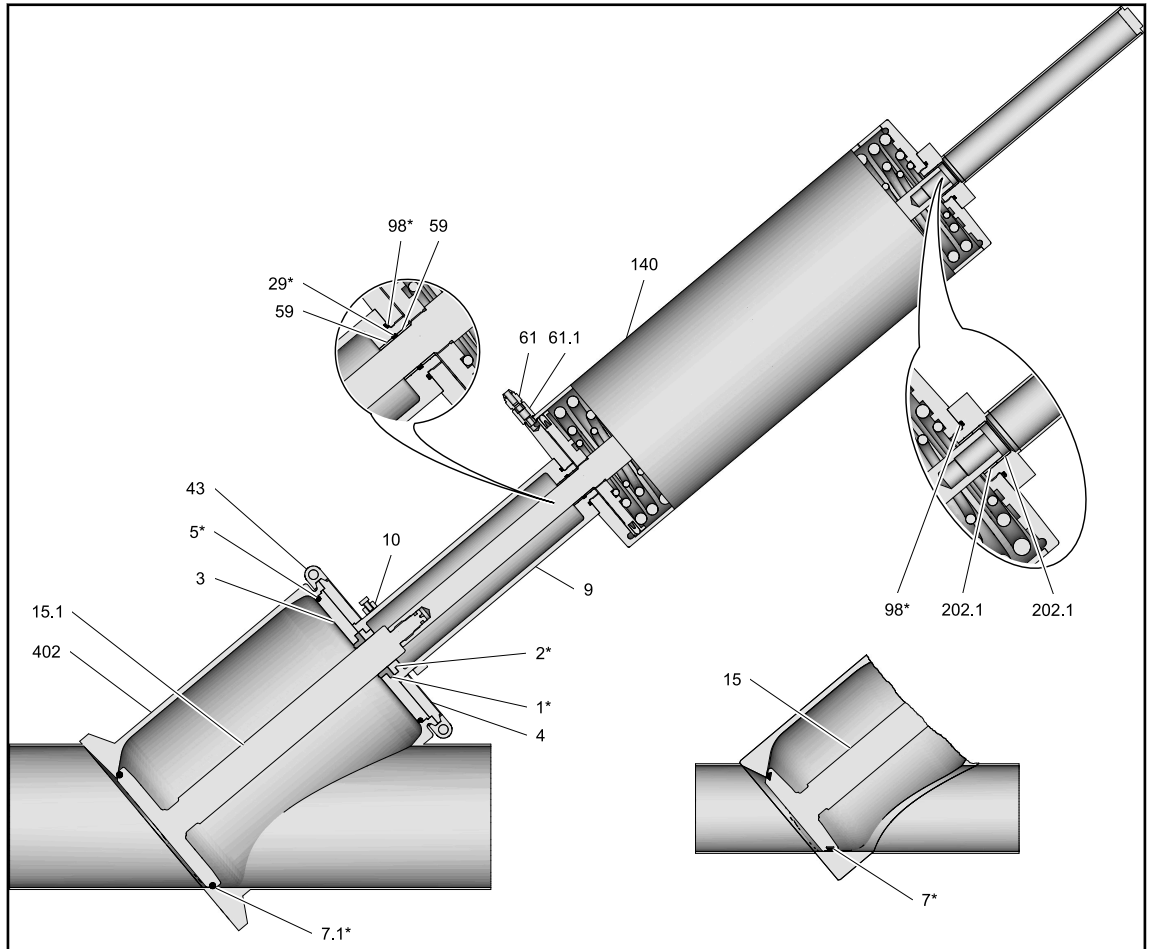
Figure 3-1 - Spare parts - Valve NI / ECO
