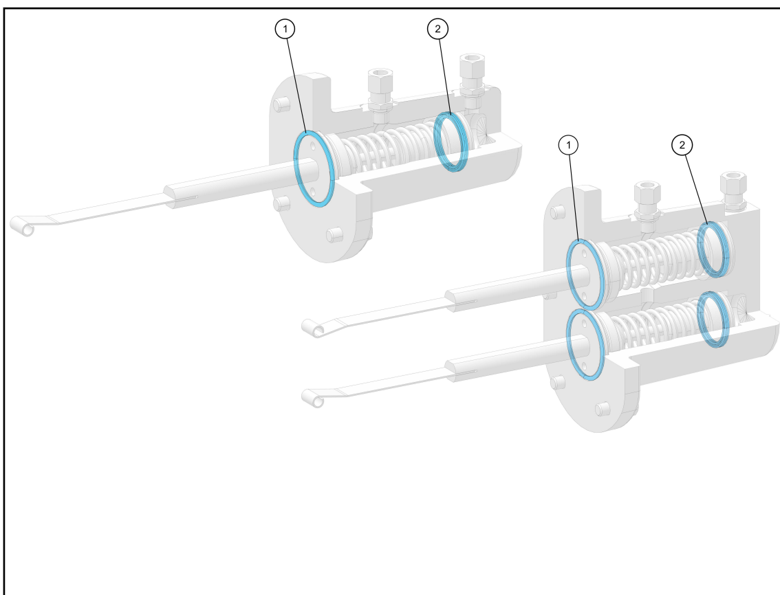
Figure 2-18 - VALVE LIFTING MECHANISM (SINGLE)
