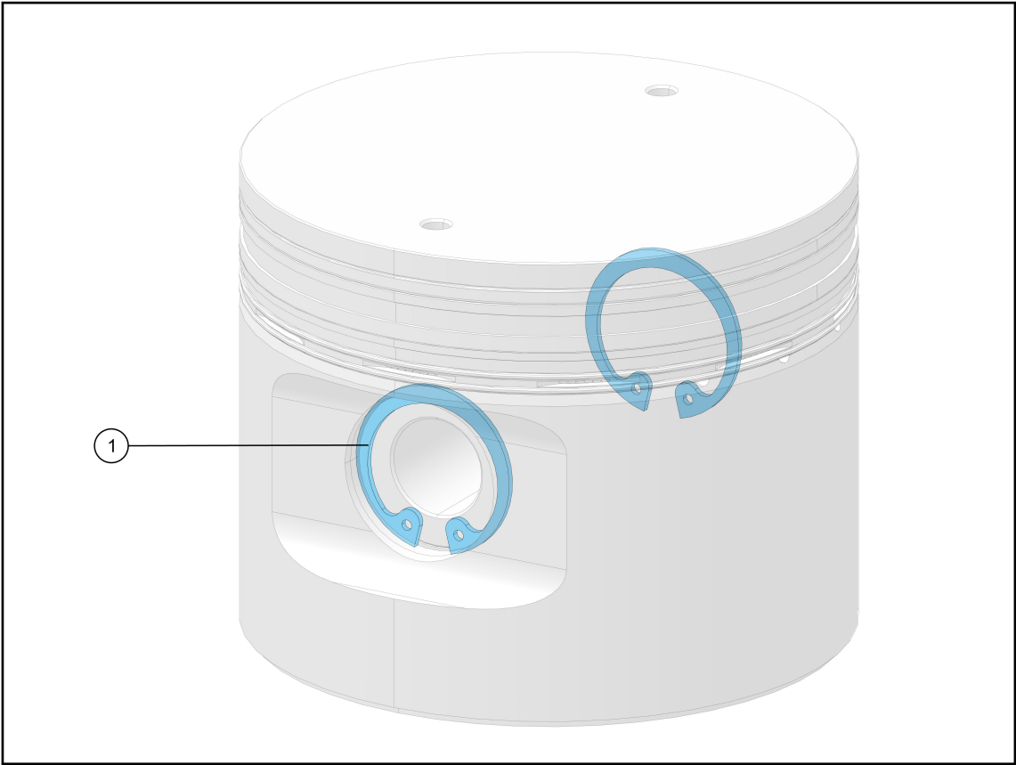
Figure 2-20 - PISTON
