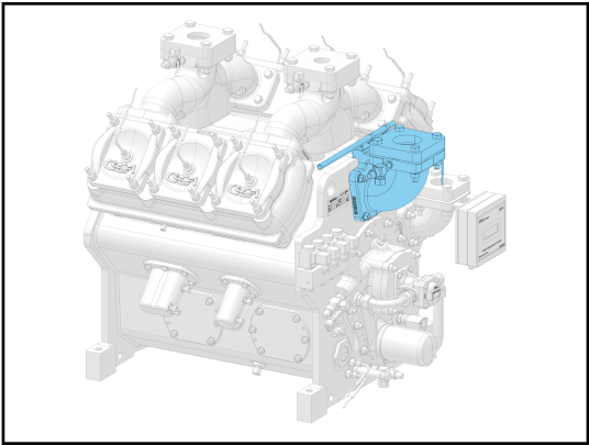
Figure 2-7 - SUCTION ELBOW
