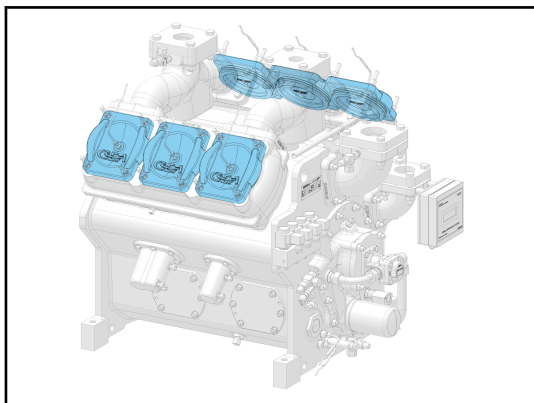
Figure 2-5 - CYLINDER COVER
