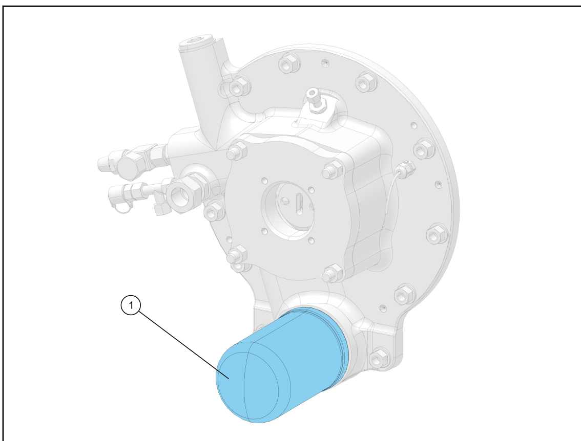
Figure 2-12 - OIL DISCHARGE FILTER
