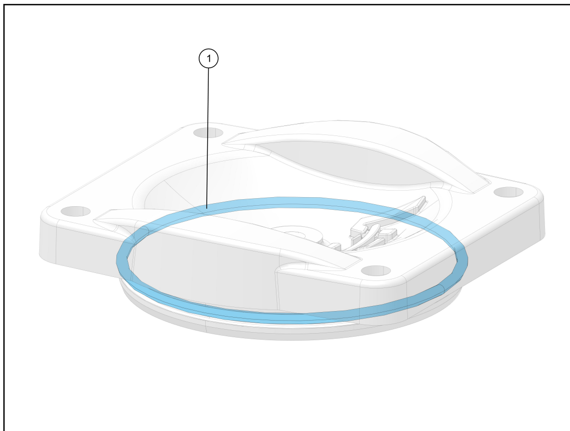
Figure 2-6 - CYLINDER COVER
