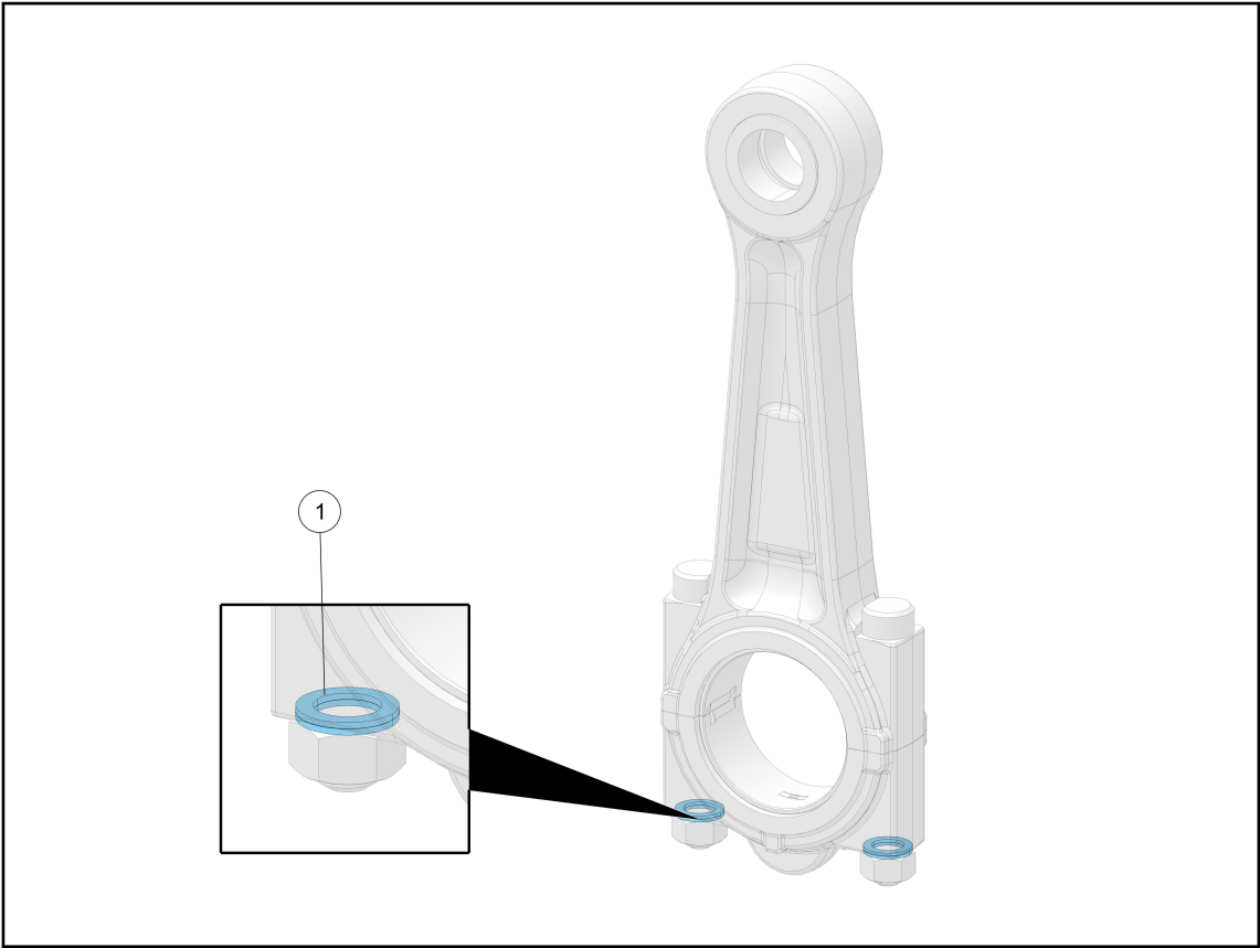
Figure 2-16 - CONROD LOCKING RING SET
