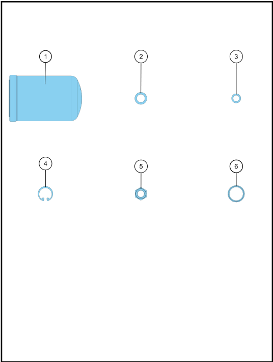
Figure 2-3 - Contents 3781018 - Service Kit B V 450(T), V450HP (2/2)
