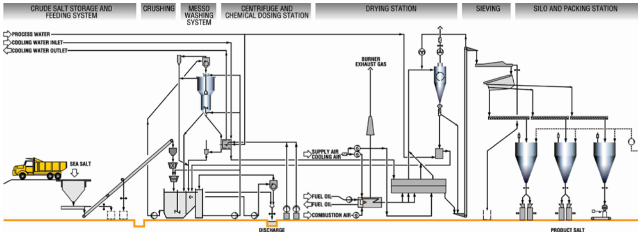
Salt wash plant
