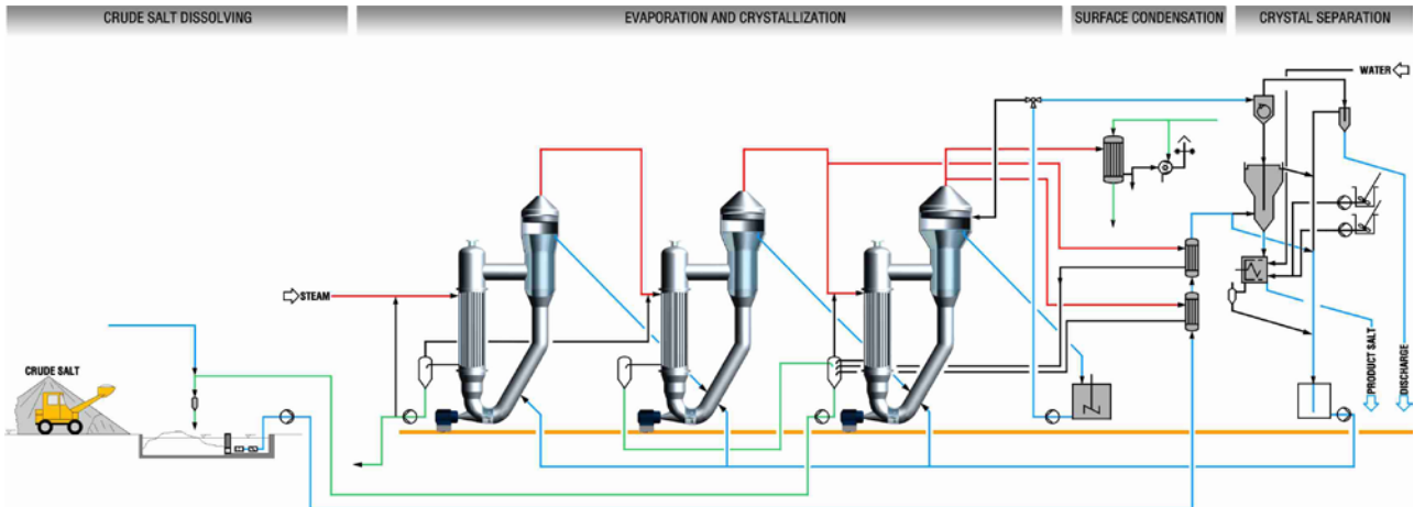
Triple-effect salt plant for recrystallization of solar salt
