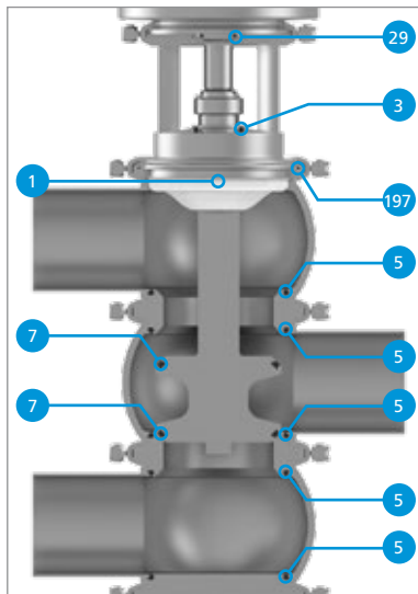
Divert valve D-tec® type W/DV with valve disc soft sealing
