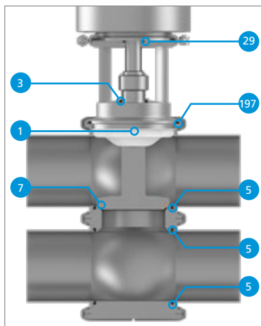
Shut-off valve D-tec® type N/DV with valve disc hard sealing
