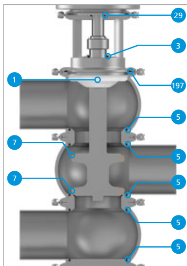
Divert valve D-tec® type W/DV with valve disc hard sealing
