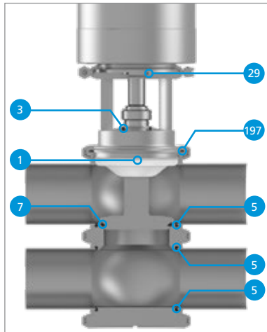
Shut-off valve D-tec® type N/DV with valve disc soft sealing
