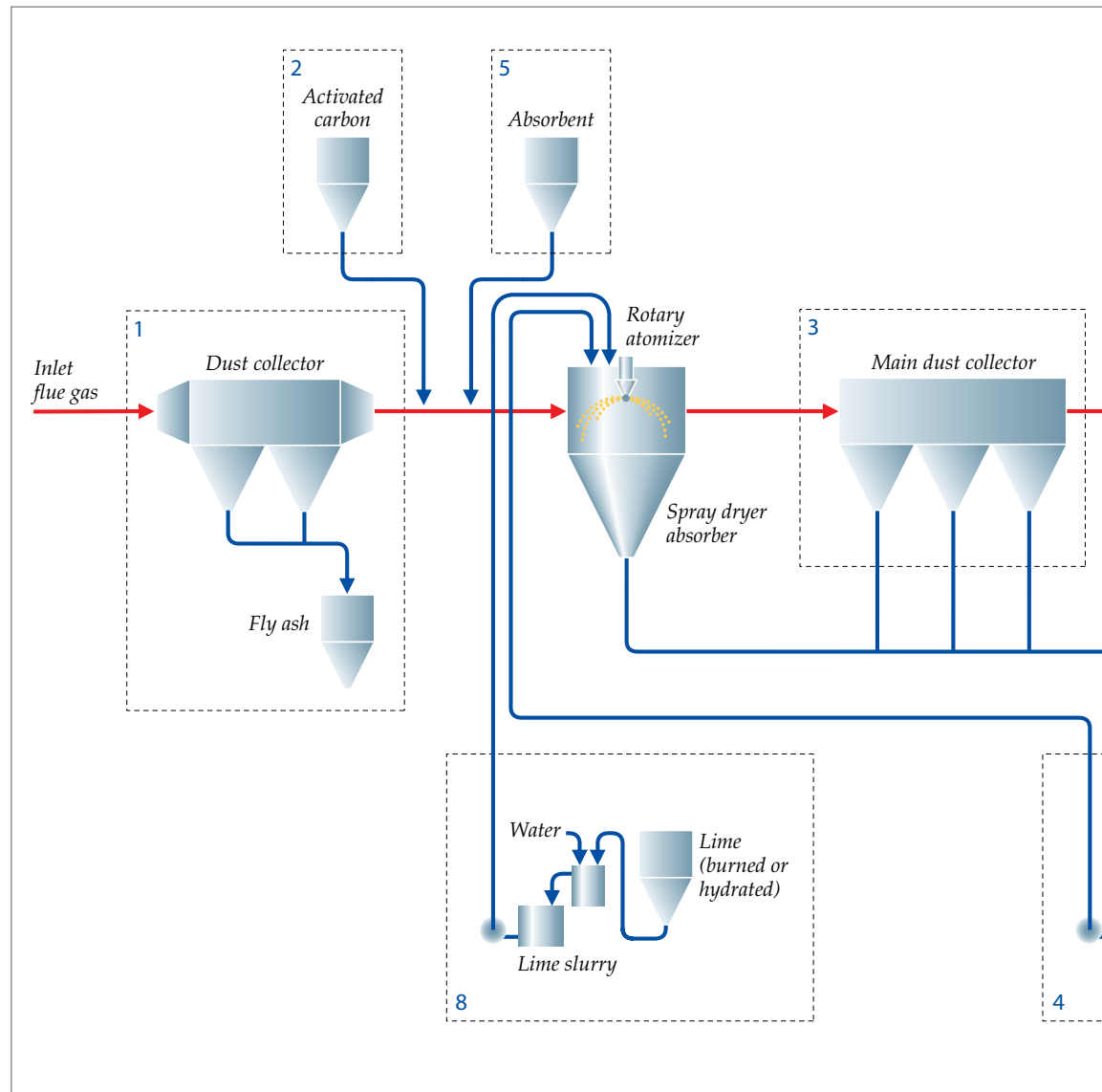
Operation of a GEA Niro SDA plant is typically handled from the central control room, without extra staffing.
