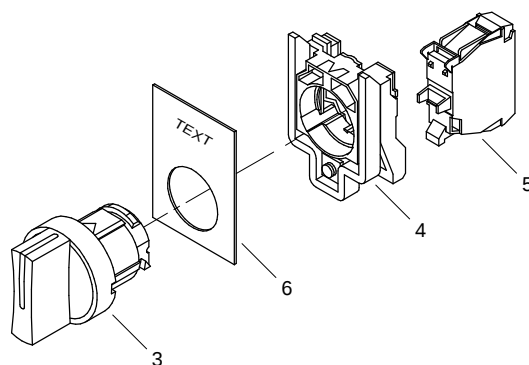
MULTI-POSITION SELECTOR
