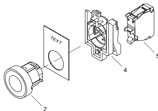
PUSH BUTTON
