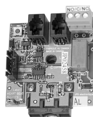
ALARM SWITCH 2005-2912-370
