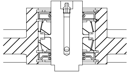
Seals installation
